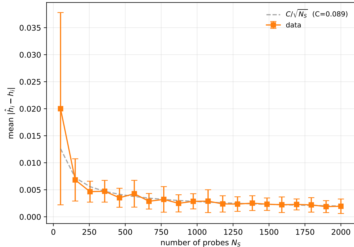
TFIM, n=10, shots=20000
