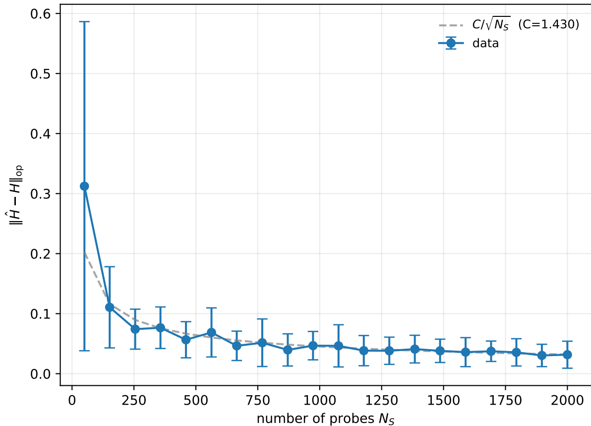
TFIM, n=10, shots=20000
